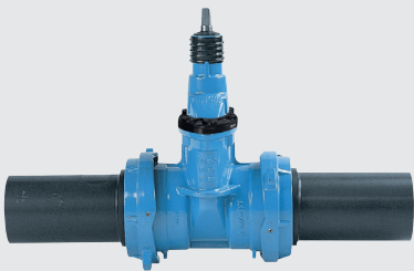
454-00 Gate valve „E3“ with steel welding ends
