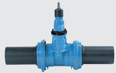
453-00 Gate valve „E3“ type D with PE fusion ends
